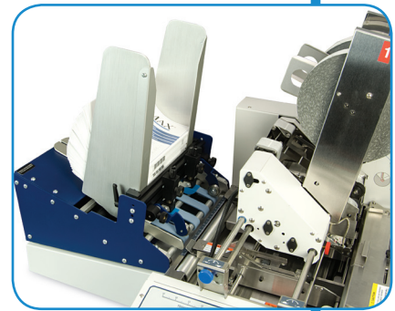
FD 282-10 Heavy Duty Friction Feeder
